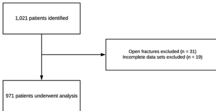
Fig. 2 – A flow-diagram of the patients identified and excluded from the AUGMENT collaborative study.
